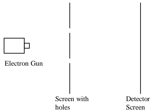
Figure 1: Classic Experiment to show basic characteristics of Quantum Mechanics
